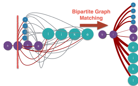
Figure 5. An example which shows how our algorithm sweeps the input image and how we construct the bipartite graph at each time slot.
