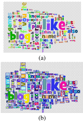
Figure 3. The letters are extracted by finding the connected components of the image. (a) The extracted letters using connected component analysis. (b) The tight bounding boxes around the letters that are used for letter size estimation.
