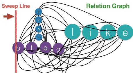
Figure 4. The word cloud relation graph is a complete graph that connects all the nodes with a similarity weight. The sweep line visits the nodes from left to right to find the words.
